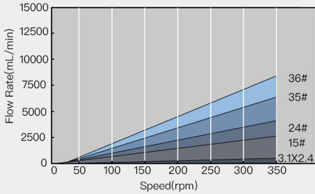
Flow Rate(0.1–350rpm)
